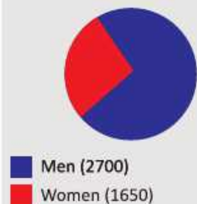
Participation Ratio in Rio Paralympics
